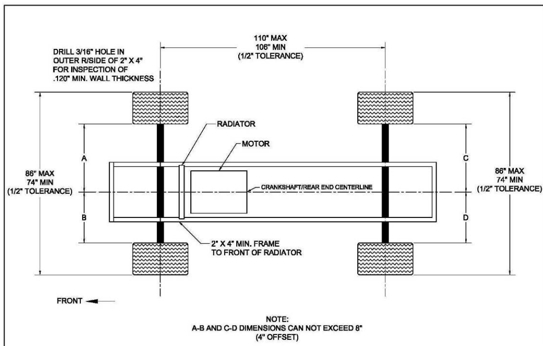
Chassis Diagram
